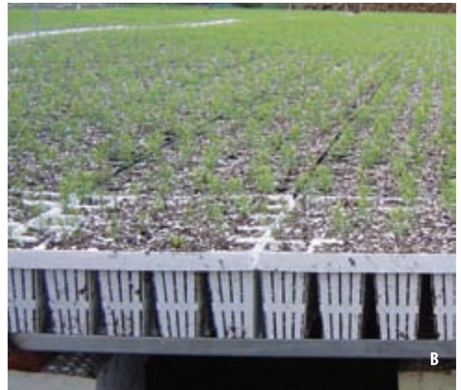
Figure 6.21 —Hardwall plastic blocks are extremely durable containers made by several manufacturers. (A) Ropak® Multi-Pots, (B) IPL® Rigi-Pots, and (C) the Hiko™ Tray System. Photos A and C by Stuewe & Sons, Inc., B by Thomas D. Landis.
