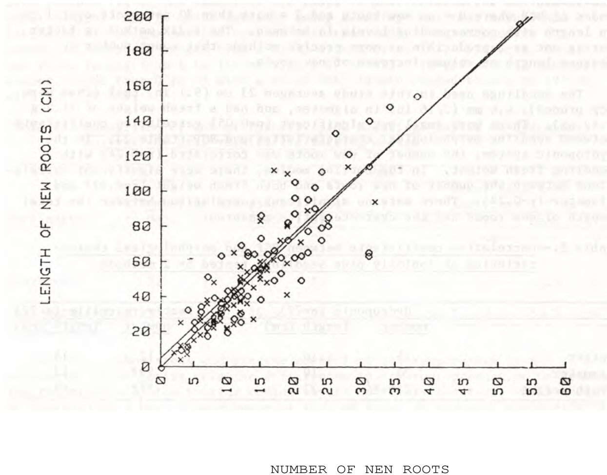
Figure 1.-- Relationship between the number of new roots greater than 1 cm and total length of new roots greater than 1 cm under both hydroponic and potting medium RGP tests. Hydroponic culture r^2 = 0.76 , peat-vermiculite r^2 = 0.80 .
