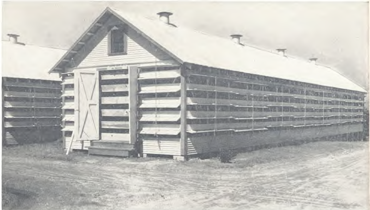
FIGURE 15.—Type of cone shed used by Region 8 of the U. S. Forest Service and by several southern States.
