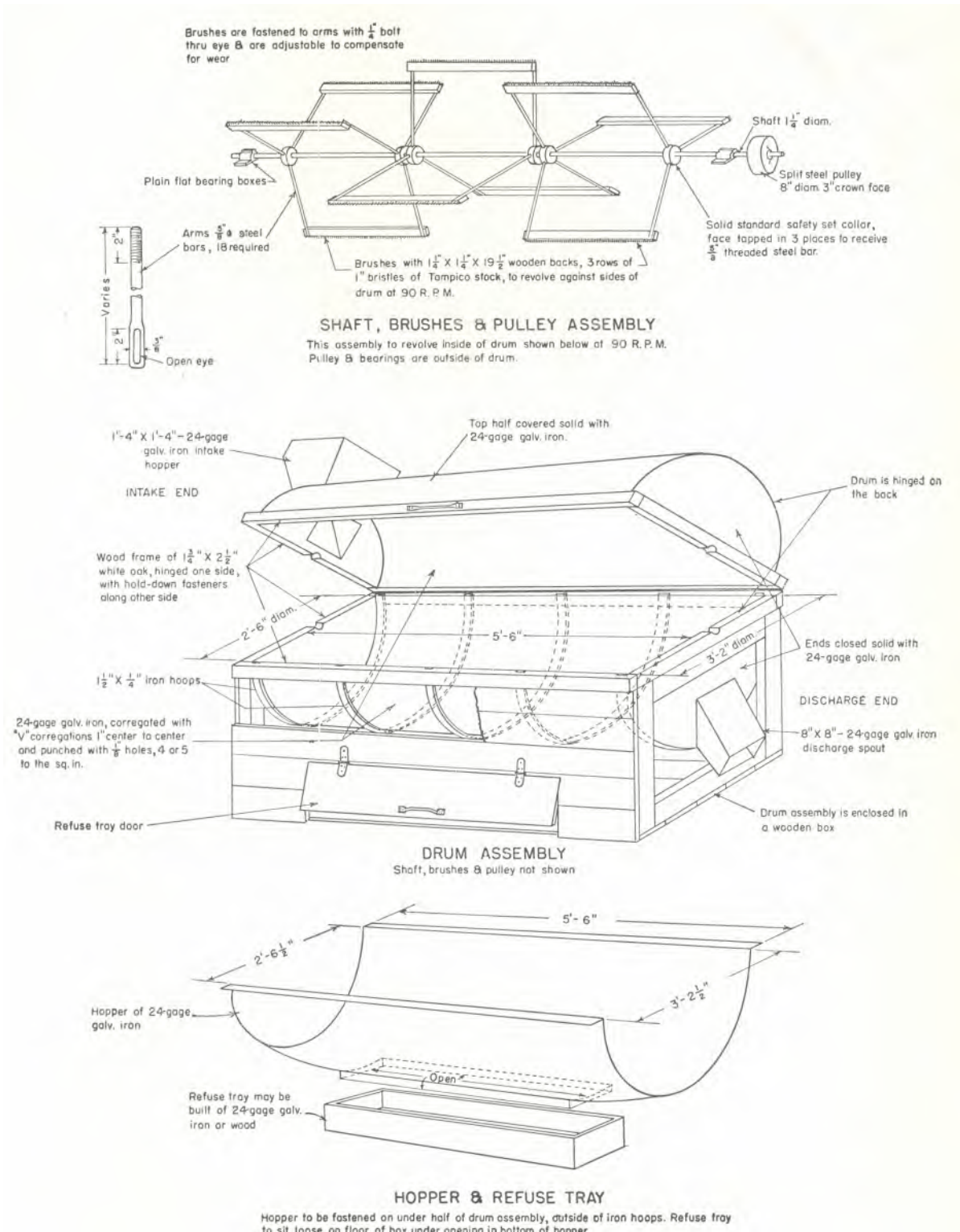
FIGURE 54.—Detailed construction of pine seed dewinger used by Region 8, U. S. Forest Service.
