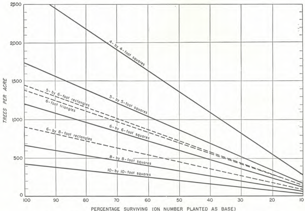
FIGURE 7.—Trees per acre at 8 initial plantation spacings and varying percentages of survival.
