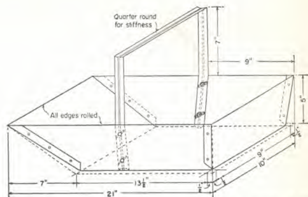
FIGURE 36.—Improved Ehrhart planting tray, made of 24-gage galvanized sheet steel and modified as suggested by Kellogg (367), used by Region 8 of U. S. Forest Service.
