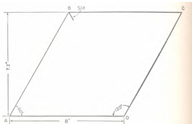
FIGURE 53.—Pattern for hardware-cloth or screen-wire cone to protect seed sown in prepared spot (498).
