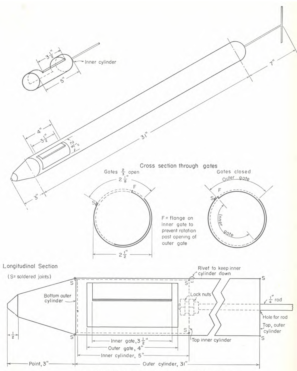
FIGURE 56.—Special probe for sampling longleaf pine seed.
