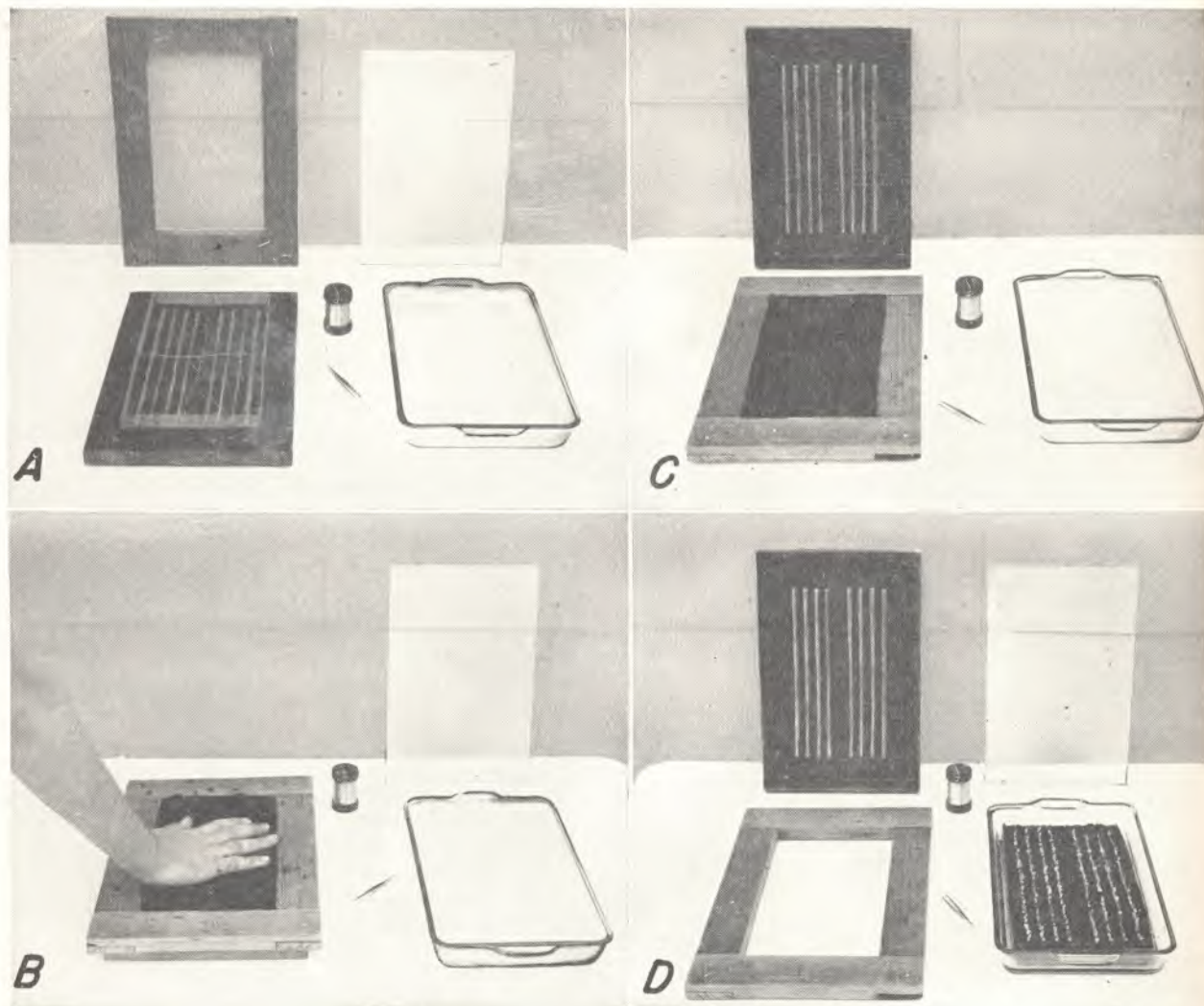
FIGURE 59.—Construction and use of peat mat for germination test. A , Mold with screen-wire collar and copper-wire cross braces in place. B , Frame in place around collar; peat being compressed to \frac{3}{4} -inch thickness. C , Mold removed from mat after inverting cover glass, frame, and mold. D , Mat in place in dish; 200 longleaf seeds in place on mat.
