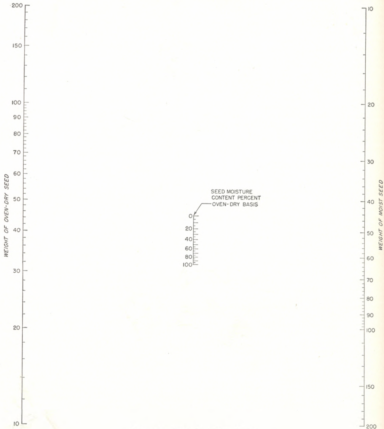
FIGURE 55.—Guide to drying of seed.
