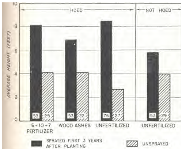
FIGURE 51.—Heights and survivals of variously hoed, fertilized, and sprayed longleaf pines, 7 years after planting. (Figures within bars are survival percents.)
