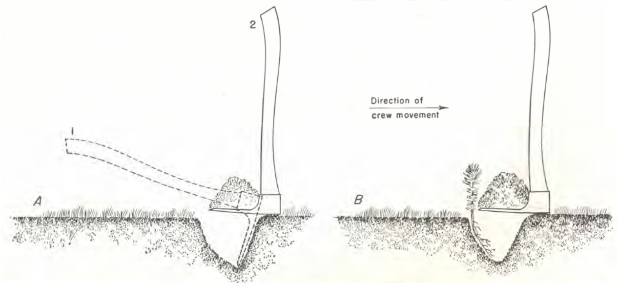
FIGURE 64.—Slit planting with mattock or grub hoe in heavier soil. A , Opening slit. B , Seedling in final position before closing slit.
