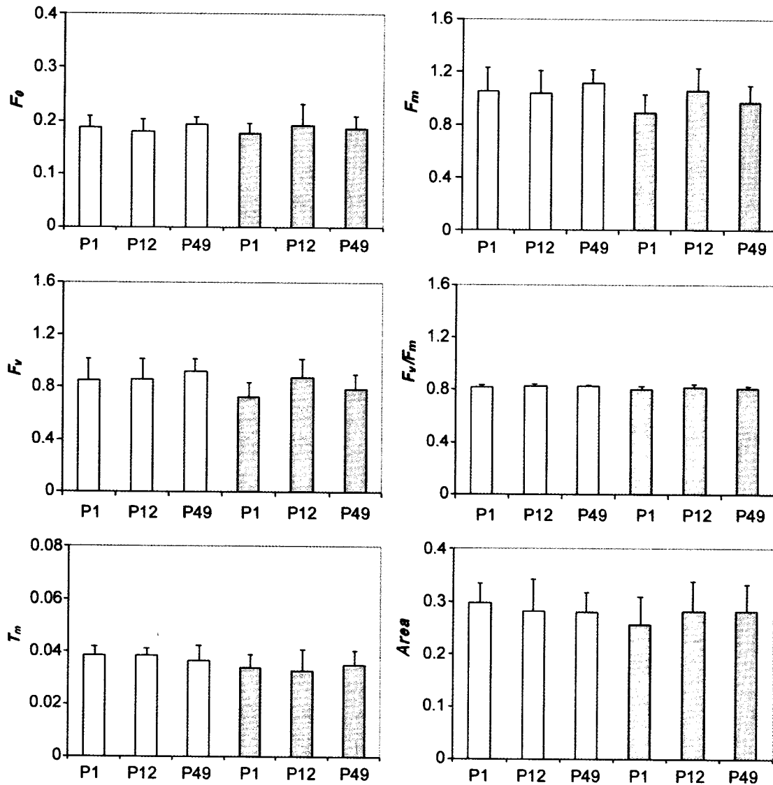
Fig. 2. Chlorophyll fluorescence parameters ( F_0 , F_v , F_m , F_v/F_m , T_m , Area) for individual provenances (means \pm SD). Unshaded columns – Vel'ký Lom trial site, shaded columns – Mútne-Zákamenné trial site.
