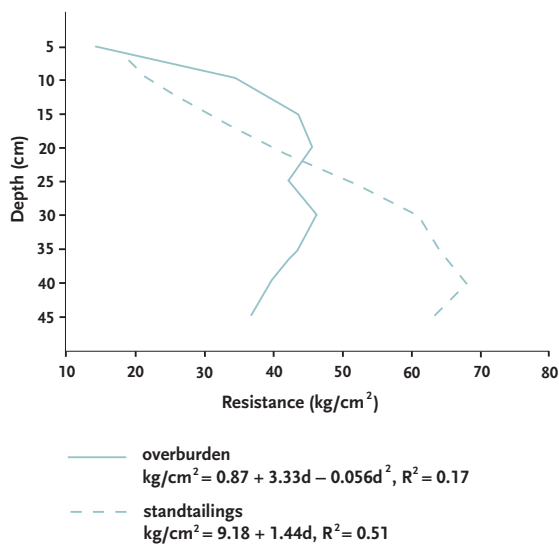
Figure 3. Penetrometer resistance over 0- to 45-cm depths on sand tailings and overburden at CF Industries phosphate mine, April 2002 (d = depth in cm). These are means over 100 observations at each site.
